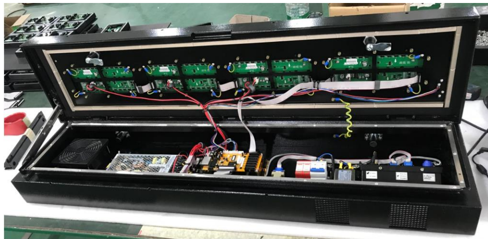
Enclosure Interior
